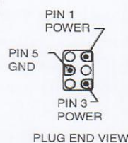
PLUG END VIEW
